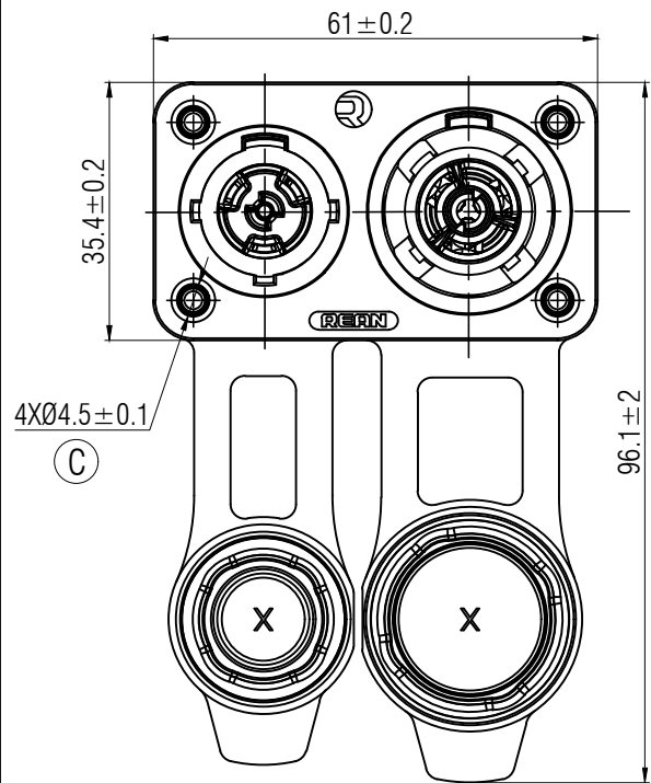
Panel cut out (Rear side)
