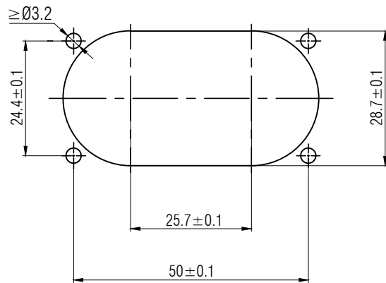
Panel cut out (Rear side)
