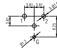
PCB-Layout (component side): ±0.1mm
