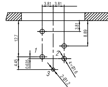
PCB-Layout (component side): ±0.1mm
