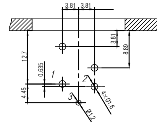
PCB-Layout (component side): ±0.1mm
