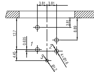
PCB-Layout (component side): ±0.1mm
