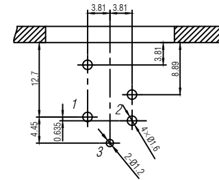
PCB-Layout (component side): ±0.1mm
