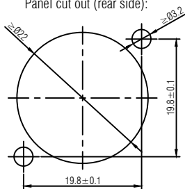
Panel cut out (rear side):
