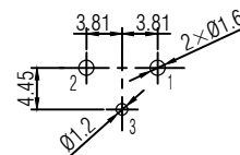
PCB-Layout (component side): ±0.1mm
