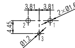
PCB-Layout (component side): ±0.1mm
