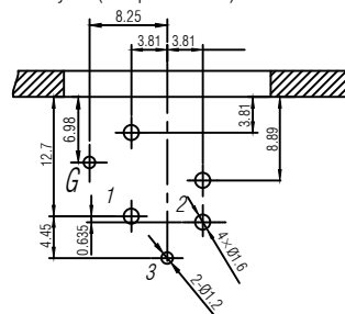
PCB-Layout (component side): ±0.1mm
