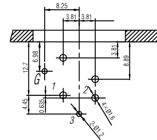
PCB-Layout (component side): ±0.1mm
