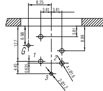
PCB-Layout (component side): ±0.1mm
