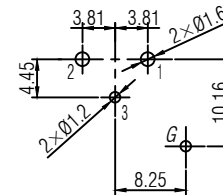
PCB-Layout (component side): ±0.1mm
