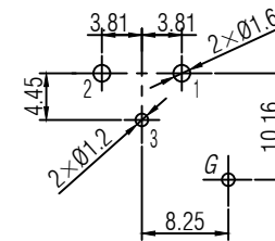
PCB-Layout (component side); ±0.1mm
