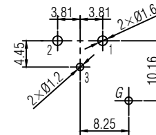
PCB-Layout (component side): ±0.1mm
