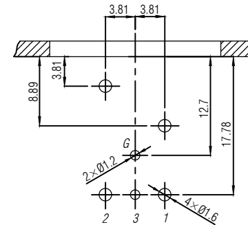
PCB-Layout (component side): ±0.1mm
