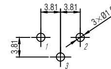
PCB-Layout (component side): ±0.1 mm
