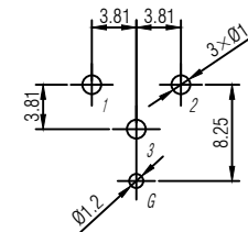
PCB-Layout (component side): ±0.1mm
