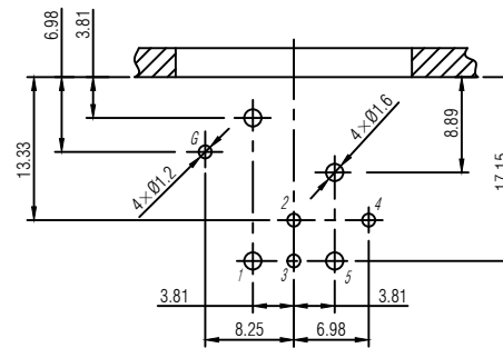
PCB-Layout (component side): ±0.1mm
